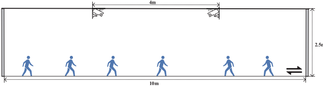
Fig. 2. The data collection scheme. Two Kinect V2 (4 meters apart) are set up in the middle of the ceiling with a -27^\circ tilt angle toward the footpath, and the distance between the ceiling and the footpath is 2.5 meters. All participants are required to perform two round-trip walks on a 10-meter footpath.
